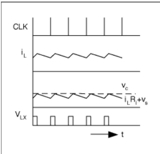
Figure 2. Current-Mode Control Waveforms
