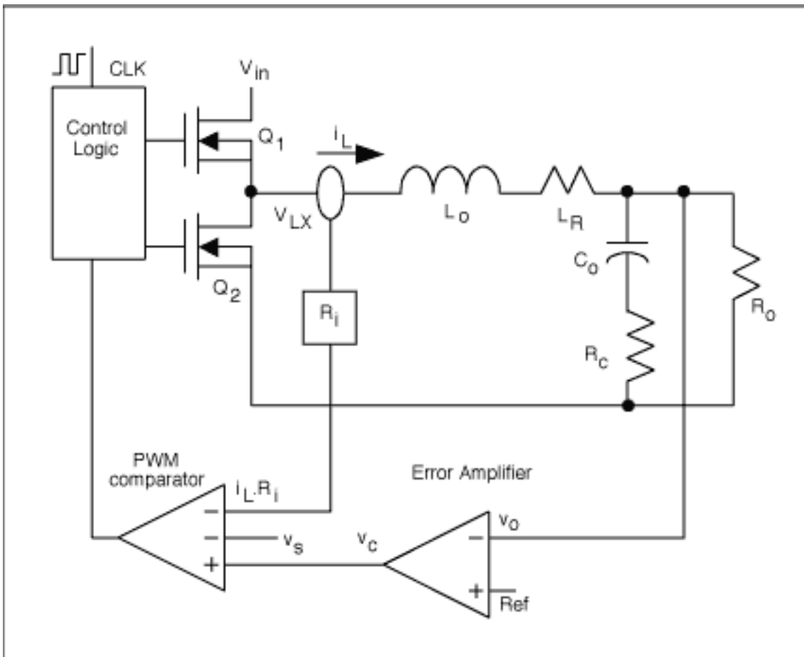
Figure 1. Peak Current-Mode Control Scheme
