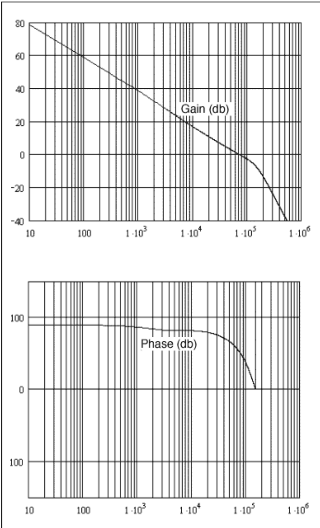
Figure 3. Control-to-Output Gain and Phase Plots from MathCad
