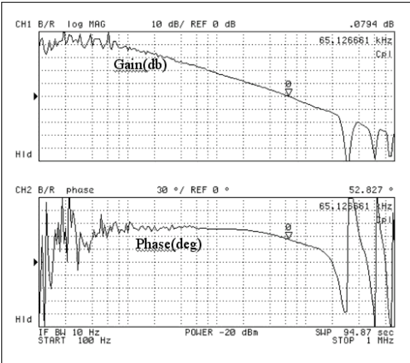
Figure 6. Measured Open-Loop Gain and Phase Plots
