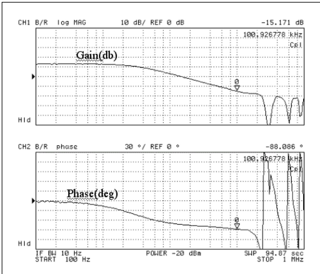
Figure 5. Measured Control-to-Output Gain and Phase Plots
